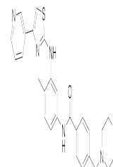
Chemical structure of Masitinib
