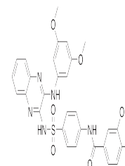
Chemical structure of SAR245409
