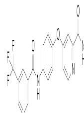
Chemical structure of SKLB 610
