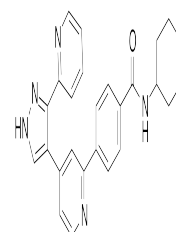
Chemical structure of GW-788388
