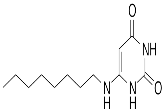
Chemical structure of GTPL-5846
