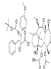
Chemical structure of Cabazitaxel N-1
