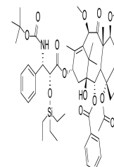
Chemical structure of 2'-TES-CABA...
