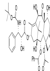
Chemical structure of 7-epi-Docetaxel
