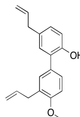
Chemical structure of 4-O-Methylhonokiol
