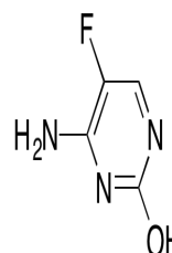
Chemical structure of 5-Fluorocytosine
