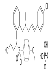
Chemical structure of KN-93
