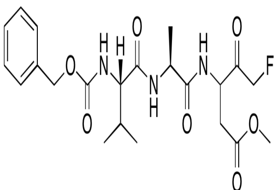
Chemical structure of Z-VAD-FMK
