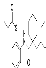
Chemical structure of Dalcetrapib
