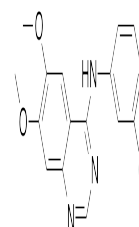
Chemical structure of AG-1478
