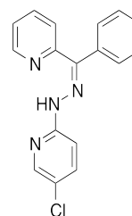
Chemical structure of Z-JIB-04
