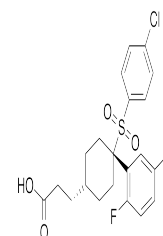
Chemical structure of MK-0752
