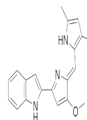
Chemical structure of Obatoclox
