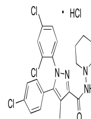
Chemical structure of Rimonabant Hydroch...
