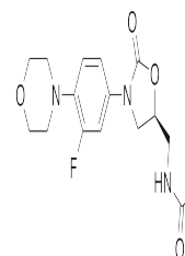
Chemical structure of Linezolid
