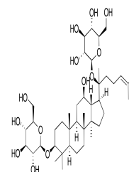
Chemical structure of Ginsenoside F2
