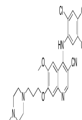
Chemical structure of Bosutinib
