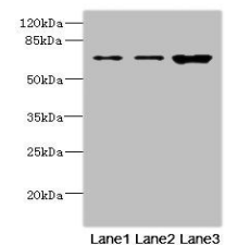
Western blot aanalysis of A549 whole cel...
