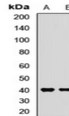
Western blot analysis of FcRn expression...
