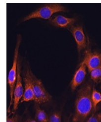
Immunofluorescent analysis of FcRn stain...
