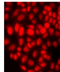
Immunofluorescent analysis of RAP80 staining...
