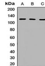
Western blot analysis of RAP80 expression...
