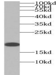
Western blot analysis of human heart tis...
