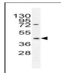
Western blot analysis of HL-60 cell line...
