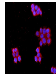
IF analysis of MPP1 using anti-MPP1 anti...
