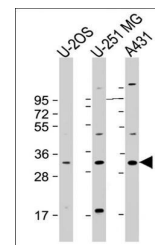
Western blot analysis of (Lane1) U-2OS w...
