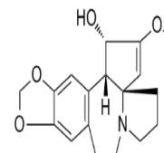
Chemical structure of Cephalotaxlen.
