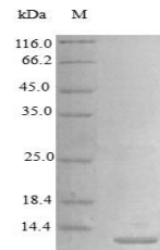
SDS-PAGE analysis of Human HBEGF protein...
