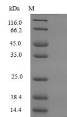
SDS-PAGE analysis of Mouse MIP3 beta pro...
