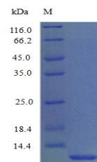
SDS-PAGE analysis of Mouse CCL3 protein ...
