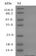
SDS-PAGE analysis of Mouse CXL10 protein...
