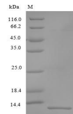
SDS-PAGE analysis of Human VCC1 protein ...
