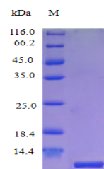
SDS-PAGE analysis of Human CXL10 protein...
