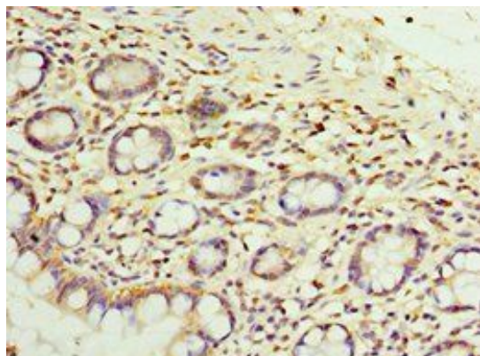
Immunohistochemical staining of human small intestine tissue using TMX2 antibody
