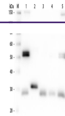
Western Blot of Anti-Rat IgG (H&L) (SHEE...
