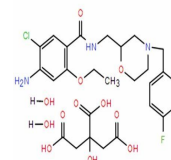
Chemical structure of Mosapride Citrate
