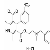
Chemical structure of Nicardipine hydroc...
