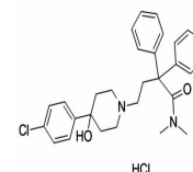
Chemical structure of Loperamide HCl
