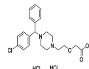
Chemical structure of Cetirizine 2HCl
