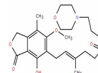
Chemical structure of Mycophenolate Mofe...
