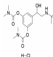
Chemical structure of Bambuterol HCl
