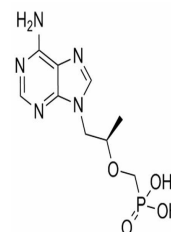
Chemical structure of Tenofovir
