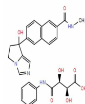
Chemical structure of Orteronel (TAK-700...)
