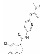
Chemical structure of SB 242084
