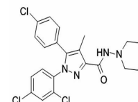
Chemical structure of Rimonabant(SR141716)
