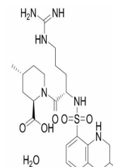
Chemical structure of Argatroban monohyd...
