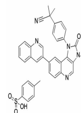
Chemical structure of NVP-BEZ235 Tosylat...
