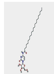
Chemical structure of Enocitabine
